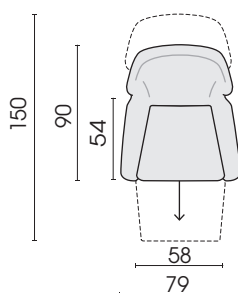
Functional chair rotatable 2 armrests 100F
