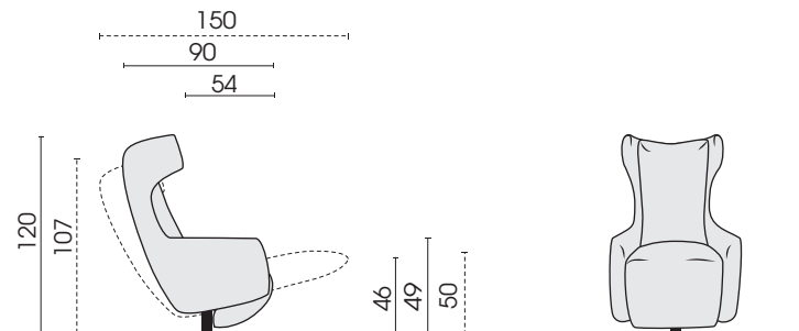
Side view, 100F
